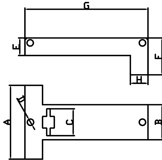
TL-Lamination Outside Structure & Size Code
