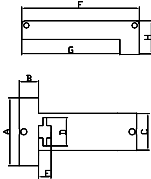
TL-Lamination Outside Structure & Size Code
